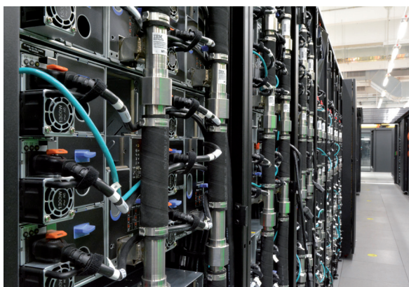
Figure 4: Rear of racks with warm water cooling.
