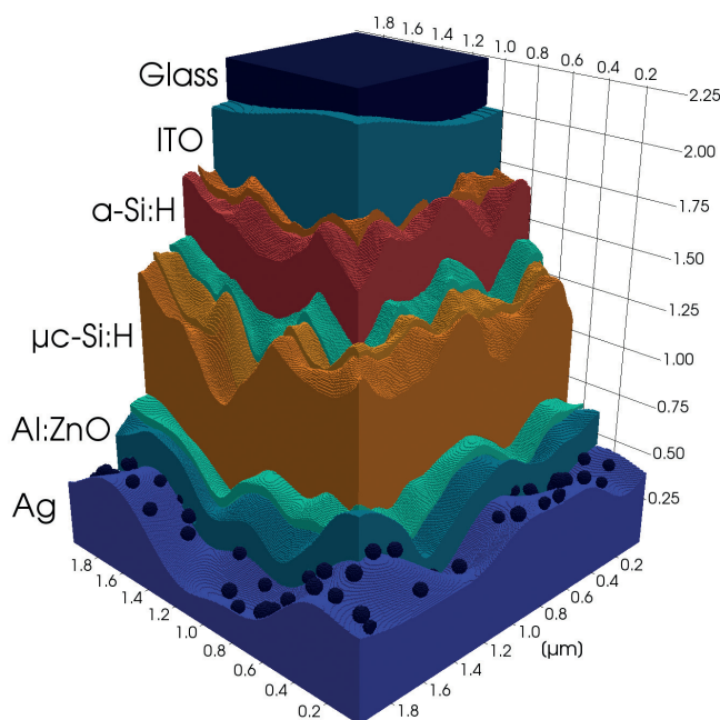
Figure 1: Cross-section of an exemplary simulation setup of a tandem thin-film solar cell. The amorphous (a-Si:H) and microcrystalline silicon ( \mu c-Si:H) layers have textured surfaces to increase the light trapping ability of the cell. SiO 2 nanoparticles are incorporated to further increase light scattering at the bottom electrode (Ag).
