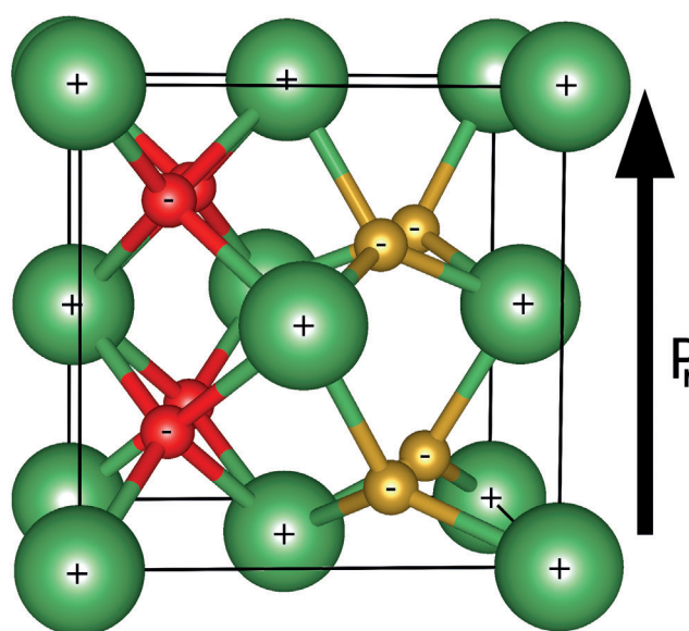
Figure 1: The ferroelectric Pca2_1 polar orthorhombic crystal structure of \text{HfO}_2 competing with monoclinic, orthorhombic, tetragonal and cubic structures. Green: metal ions, Red: oxygen ions, Gold: stable asymmetric positioned oxygen ions responsible for ferroelectricity. Arrow marks the polarization vector P_r .
