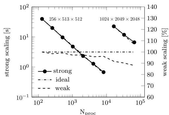
Figure 1: Strong and weak scaling of the semi-implicit Runge-Kutta solver implemented in DINO [5] for two different cases.
