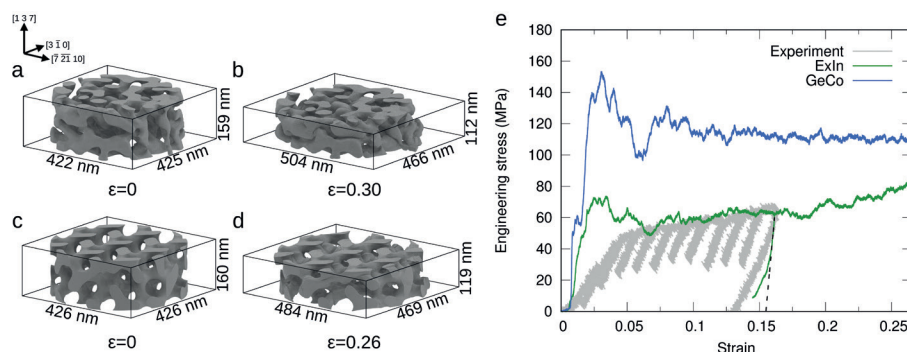
Figure 1: Experimentally informed (ExIn, top) and geometrically constructed (GeCo, bottom) NPG configuration before (a,c) and (b,d) after 0.30 and 0.26 compressive strain. e) Comparison of the stress-strain curves of MD simulations on ExIn and GeCo and experiment.
