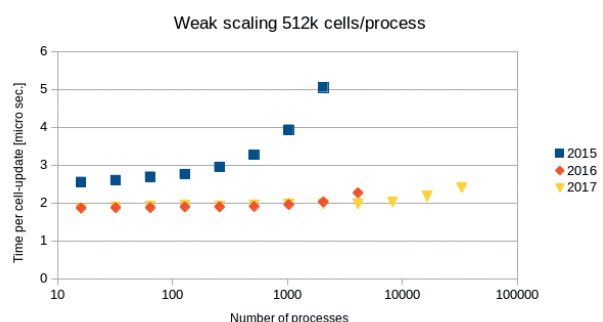
Figure 1: Improvement of parallel weak scaling performance expressed as time per cell-update as function of number of MPI processes. The problem size was set at 512 \times 10^3 cells per MPI process. The tested architecture is SuperMUC Phase 1 (Intel Sandy Bridge).
