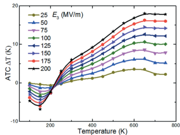
Figure 5: Adiabatic temperature change in PMN 0.4 PT 0.6 in applied electric field. This electrocaloric effect can be used for solid state refrigeration and energy scavenging from excess heat.
