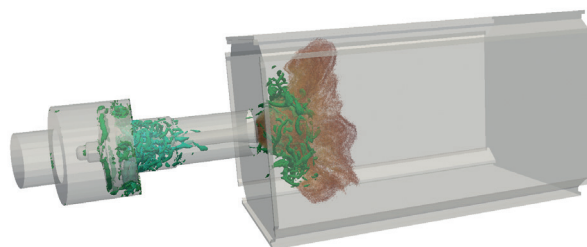
Figure 1: Snapshot of the compressible LES computation for the confined swirl combustor. The turbulent structures (green iso-surfaces) that are generated across the radial swirler impinge on the flame front (orange iso-surface) and cause thereby turbulent combustion noise.
