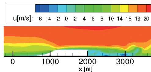
Figure 5: Velocity distribution in complex terrain
