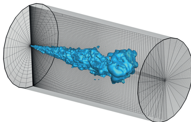
Figure 2: Typical mesh for single-injector simulations.
