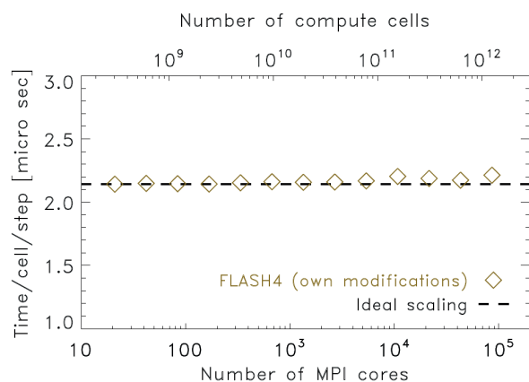
Figure 1: Weak scaling of the customized version of the FLASH code, used during the SuperMUC scale-out workshop on Phase 2 in 2015. The diamonds indicate the scaling tests of the FLASH code, while ideal scaling is represented by the dashed line.
