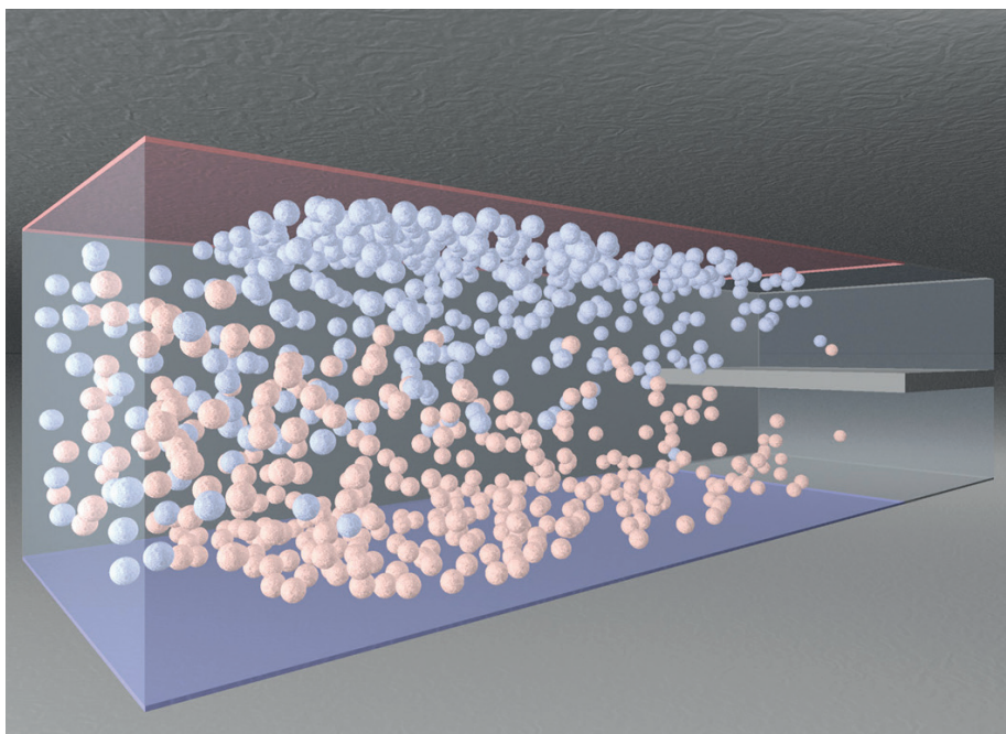
Figure 3: Bisecting micro-channel: separation of oppositely charged particles with a radius of 60µm in fluid flow.
