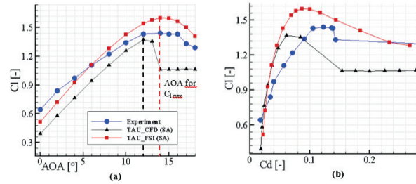
Figure 3: (a) Lift coefficient Cl as a function of the angle of attack (AOA) for the experiment, the rigid TAU-investigated case and the FSI computations; (b) Lift coefficient as a function of the drag coefficient for the same cases.
