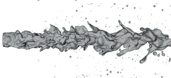
Figure 1: Gas-liquid surface of a spatially developing round jet with Re=5,000 and We=2,000 .
