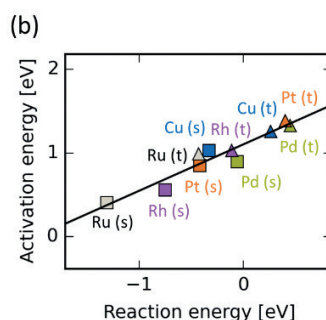
Figure 1: (a) DFT-calculated energies and structures of the initial, transition and final state for the dissociation of a water molecule on a terrace site of a Rh(211) catalyst. (b) Scaling relation between the activation energy and the reaction energy of the water dissociation step illustrated for terrace (t) and step (s) sites on the (211) facet of several transition metals. Based on data from Ref. [1].
