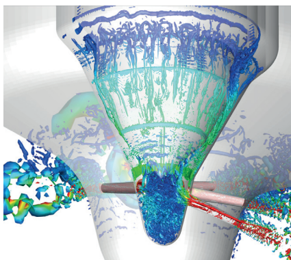
Figure 3: Coherent vortical structures during the main injection phase colored by velocity in the half-domain.
