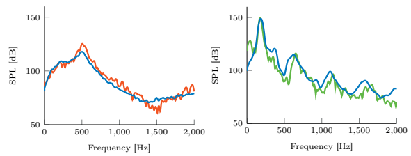
Figure 5: Measured (blue) and computed (red / green) sound pressure spectrum within the confined combustor geometry. Left: stable working conditions. Right: unstable working condition. Reproduced from [3].
