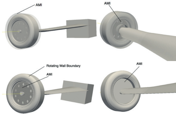
Figure 2. AMI of two different methods with sliding mesh In the next step, the full car simulations with DDES and sliding mesh is studied, in order to study the influence of wheel parameters, based on the DoE plan, there are 25 configurations covering 15 parameters of a automotive wheel, as seen in Fig.3.
