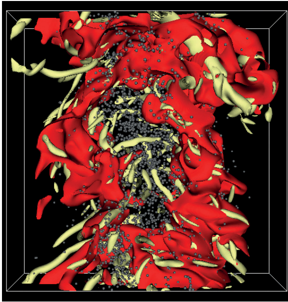
Figure 1: Spray combustion in TEJ; the gray spheres represent the liquid droplets (size is multiplied by factor of 5 for visualization), the yellow iso-surface is the Q-criterion showing the main turbulent structures, and the red iso-surface represents the temperature ( T = 1800 K)
