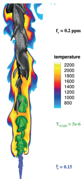
Figure 2: Instantaneous APDF/LES results.
