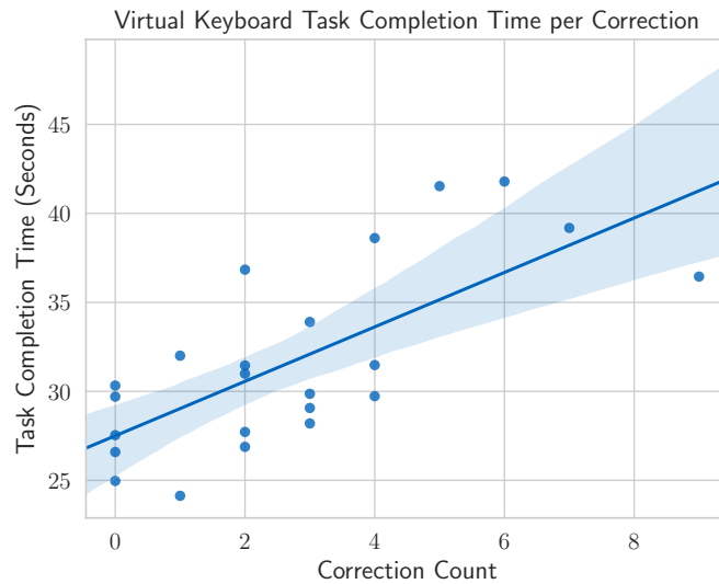
Figure 5.2.7.: A scatter plot of the time it took to complete the virtual keyboard task per correction count. The line visualizes the linear regression with a 95% confidence interval. The more corrections were made, the longer participants took to complete the task.
