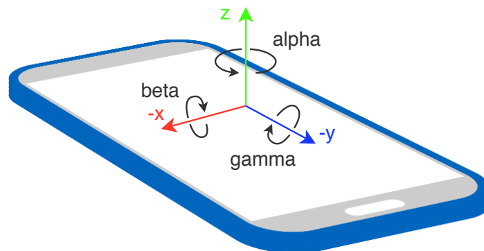
Figure 3.3.1.: The specification of the orientation values visualized. The x and y axes are inverted for the sake of clarity in this graphic. The arrows indicated the direction where Euler angles increases. alpha , beta and gamma describe the three rotation angles.
