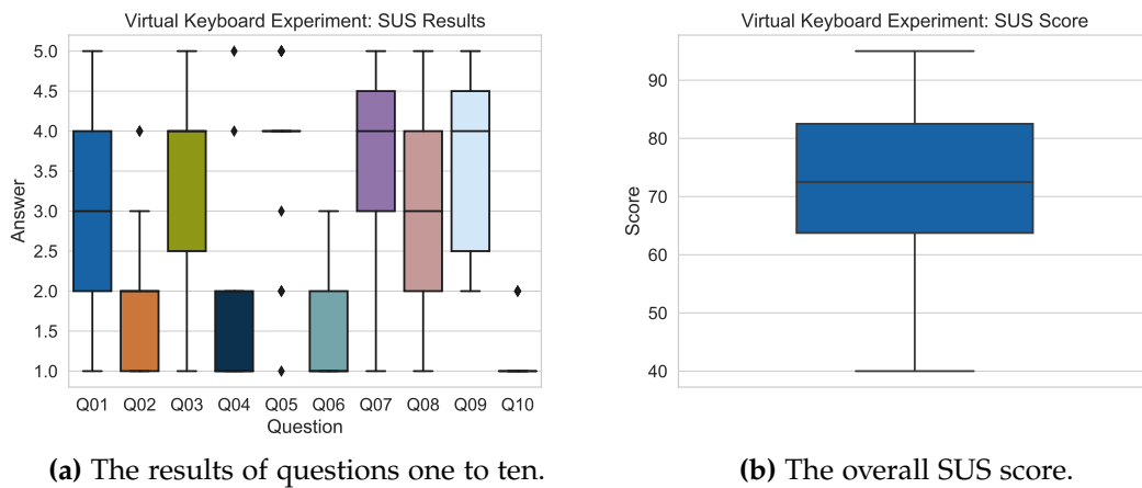
Figure 5.2.8.: The results of the SUS user study for the virtual keyboard experiment.
