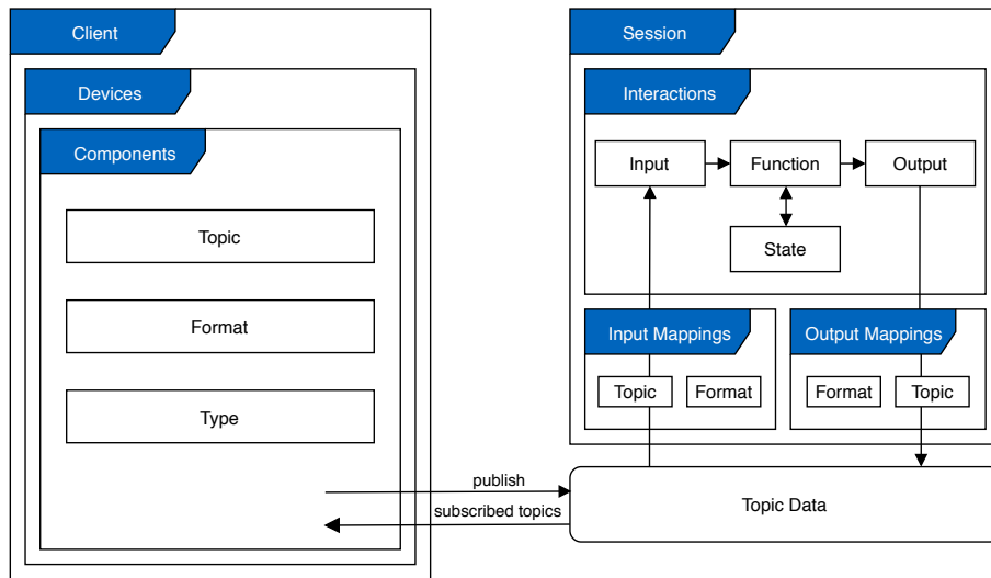
Figure 3.1.2.: The interaction processing overview. This graphic gives a rough overview of the dataflow when using an Interaction. The diagram was created with the help of Sandro Weber. Rectangles represent entities, rounded rectangles represent data, and arrows represent the data flow. The flow is described in detail in Subsection 3.1.1. Client components are on the left portion of the figure, while components running on the server are located on the right side.
