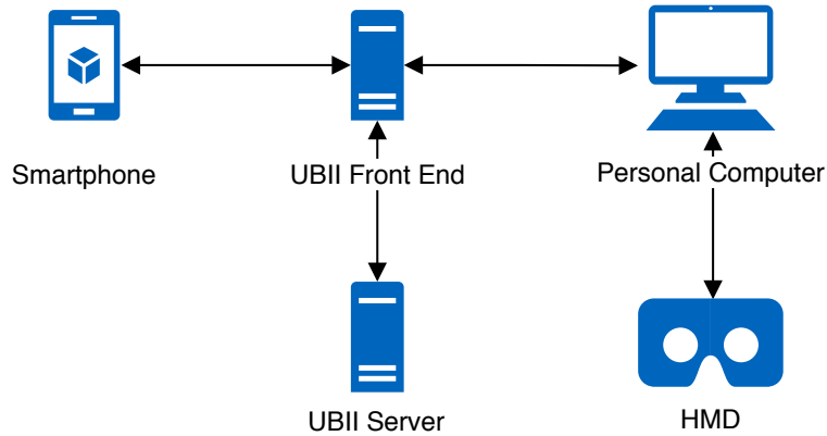
Figure 3.4.1.: This diagram shows the simplified architecture of the complete system. An arrow means that the connected applications exchange data. Multiple instances of the smartphone or front end are combined into one diagram entity. The web server, serving the front end, is hidden for the sake of simplicity.
