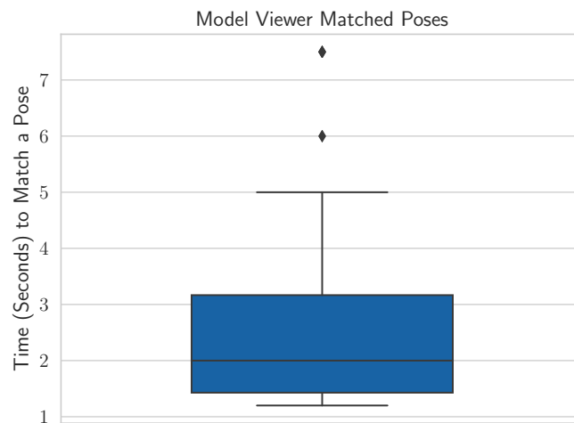
Figure 5.2.3.: The time in seconds it took to match a correct pose in the model viewer experiment.
