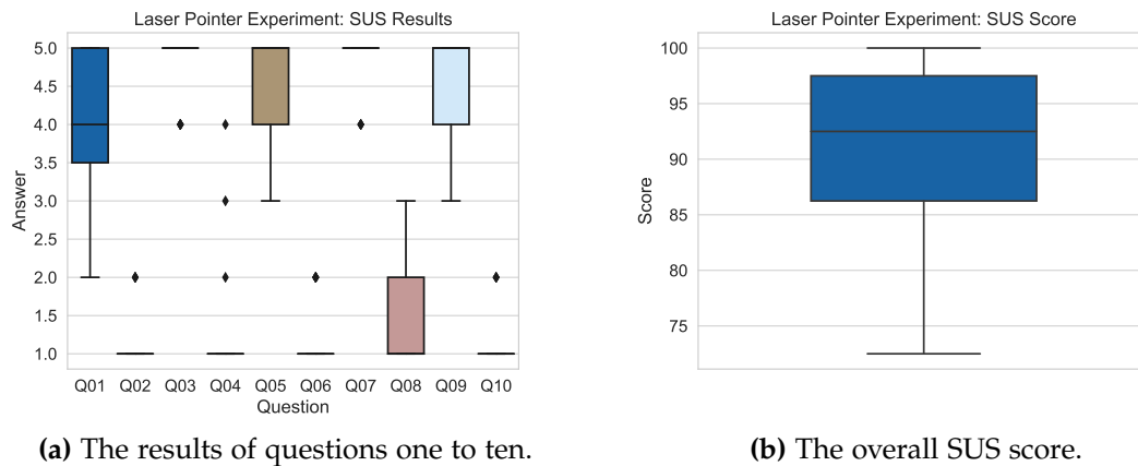
Figure 5.2.6.: The results of the SUS user study for the laser pointer. Ignoring a few outliers, participants clearly agree on most SUS questions, as seen in Figure 5.2.6a.
